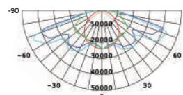
Beam Angle: 170.7°
