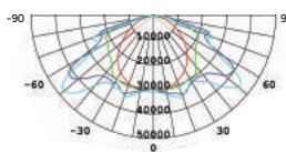
Beam Angle: 136.0°
