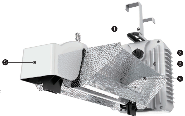
Nobel Pro Fixture Greenhouse Bracket (SKU#94132)
