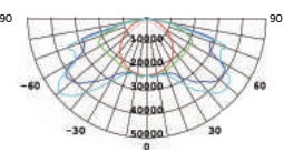
Beam Angle: 142.0°
